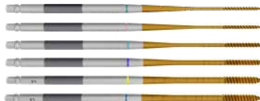
Cannulated Tap, Ø4.5mm 6300-71-45
