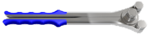
French Rod Bender 6000-16-S
